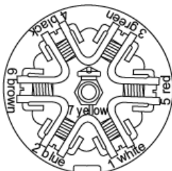
Fig. 3.2 7-way trailer plug Car end, rear view
